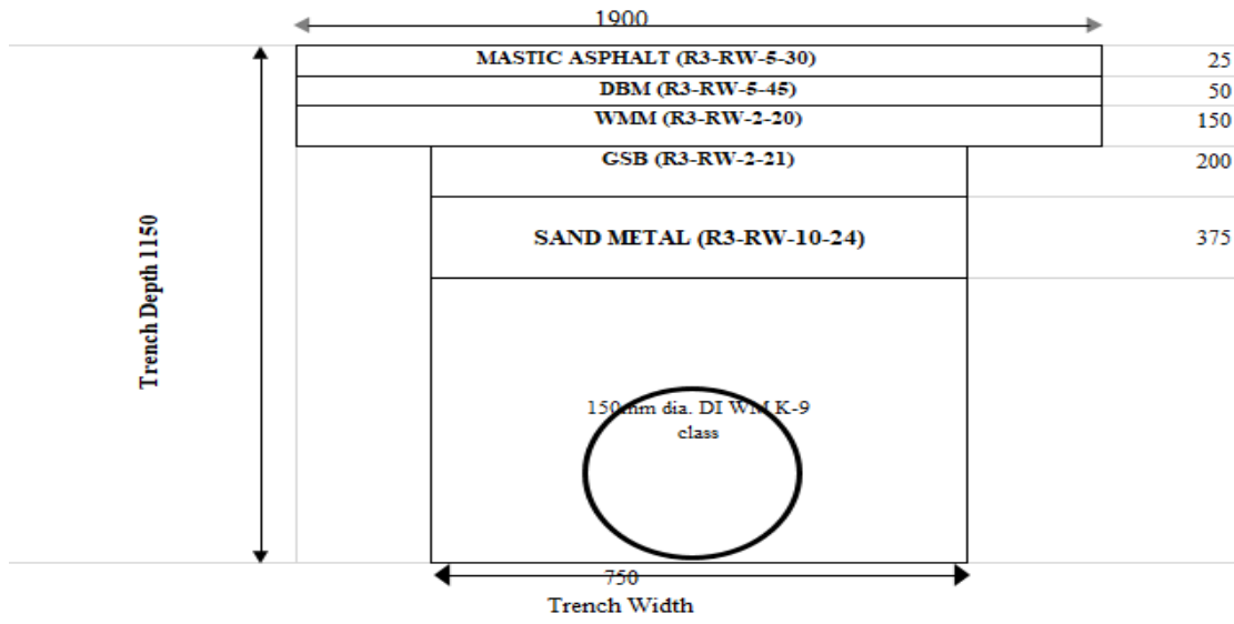
Typical Cross Section of Trench For Laying of 150 mm dia. DI WM in Mastic Asphalt
